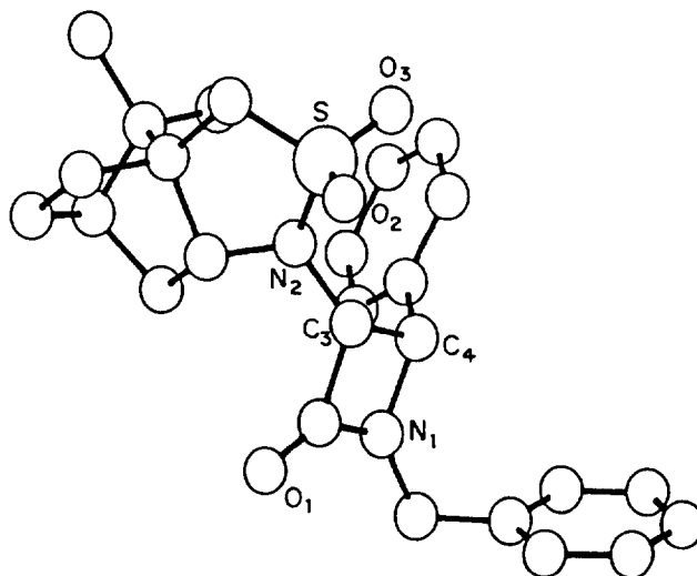
Fig. 1. Pluto diagram of 6d
